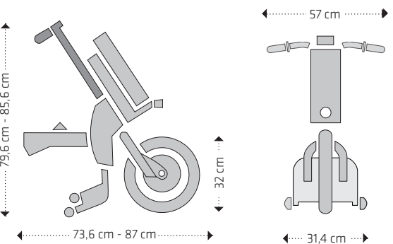
FOLDED OUT
