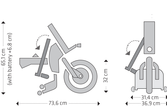
FOLDED IN
